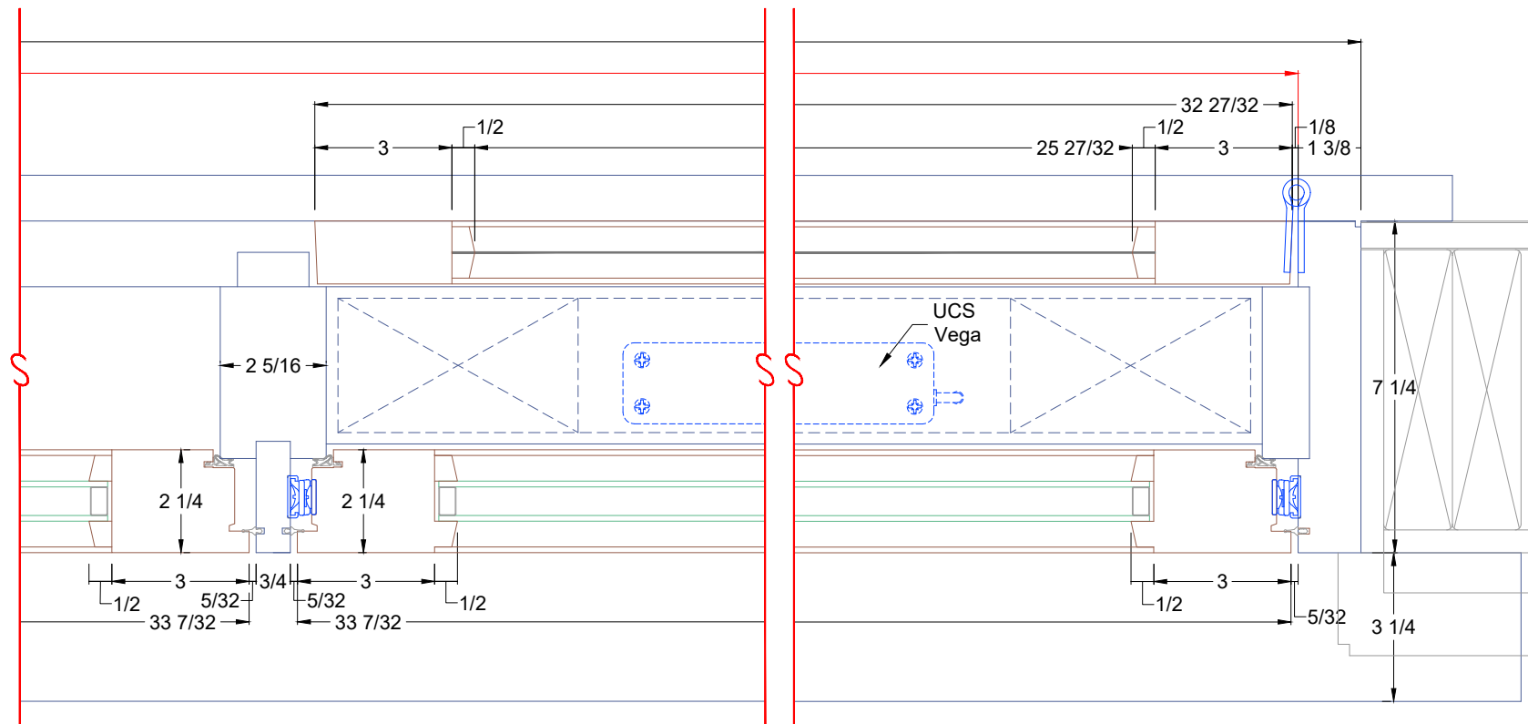
B Detail at plan view Scale: 3" = 1'
