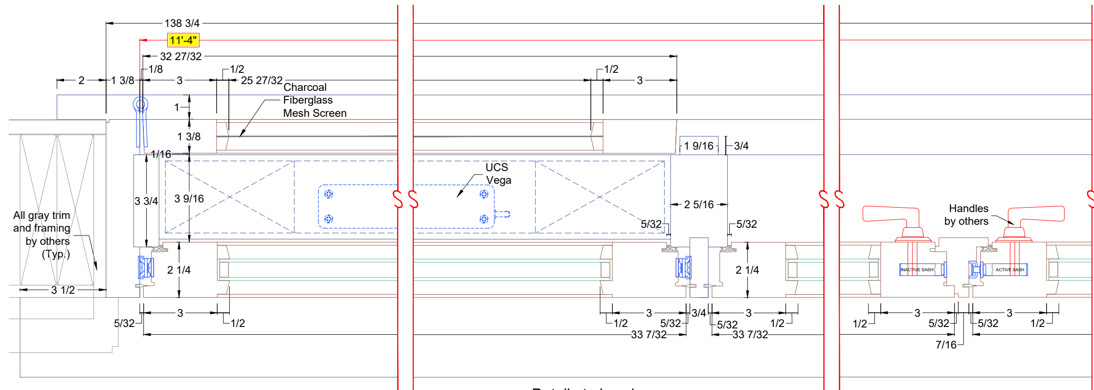
A Detail at plan view Scale: 3" = 1'
