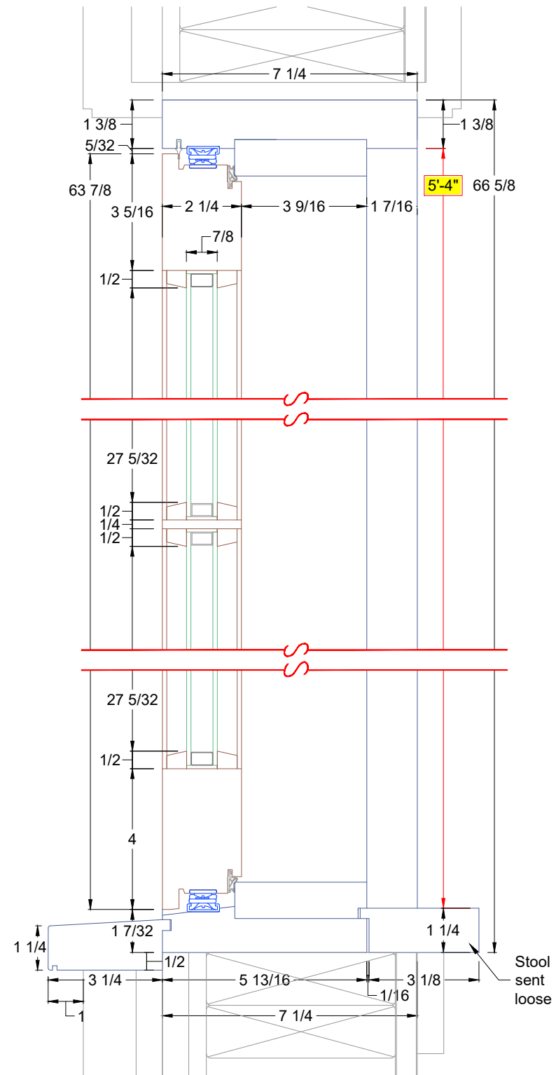
B Detail at head and sill, Casement Scale: 3" = 1'
