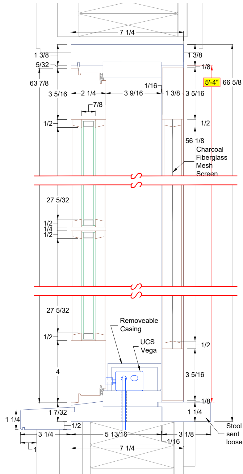
A Detail at head and sill, Awning Scale: 3" = 1'
