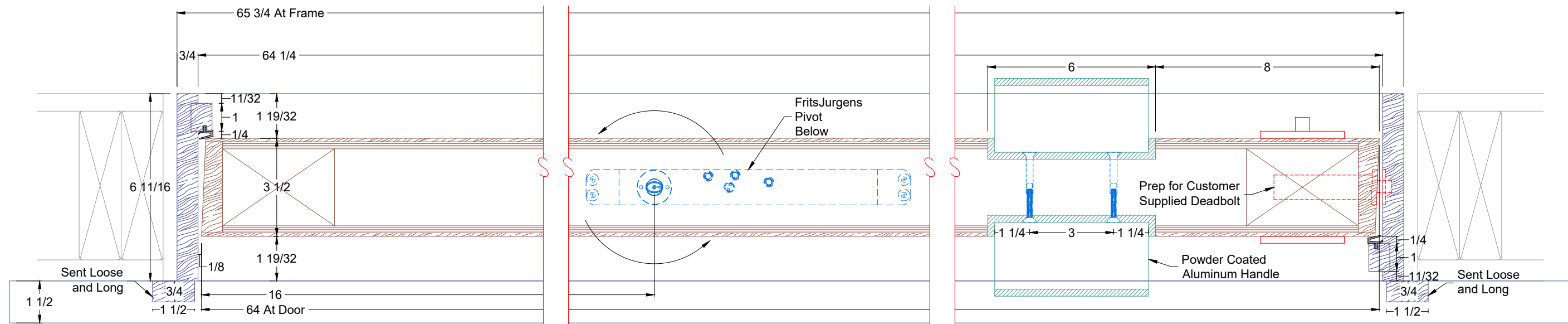
A Detail at plan view Scale: 3" = 1'
