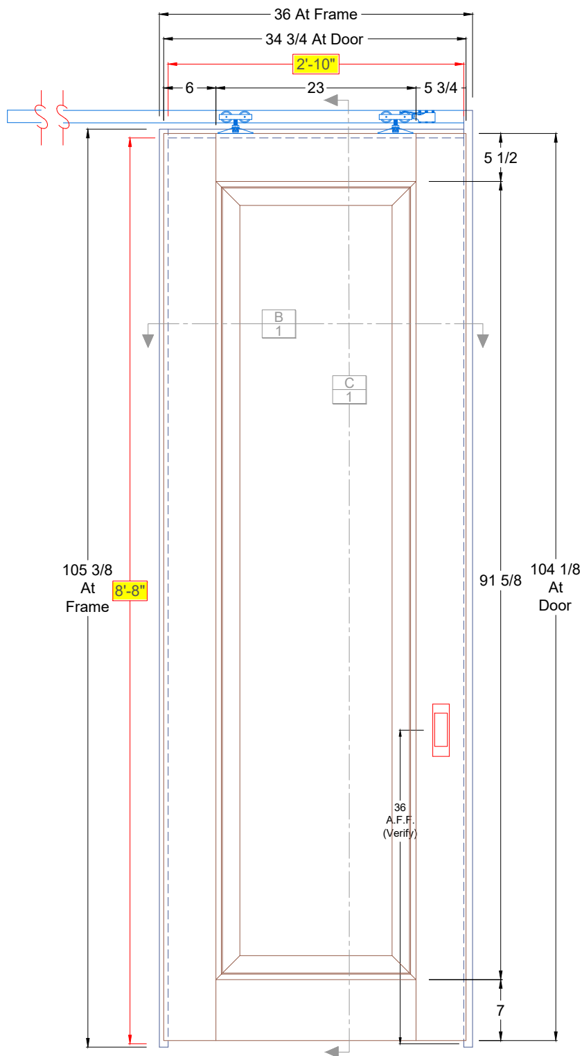
A Elevation at unit Scale: 3/4" = 1' Make 1 single as drawn
